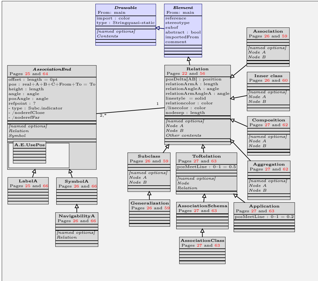
Figure 3: Relation commands in uml.sty.
