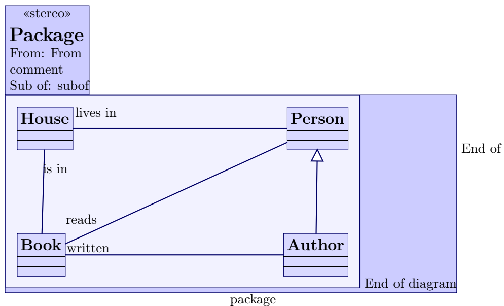
Figure 11: Example of package
