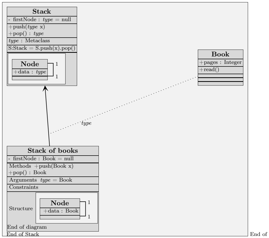
Figure 10: Example of abstraction and application
