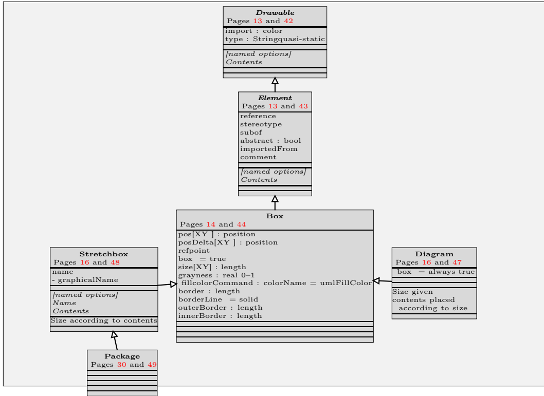
Figure 1: Main commands in uml.sty. This and the following class diagrams work as a short-form documentation of uml.sty.
